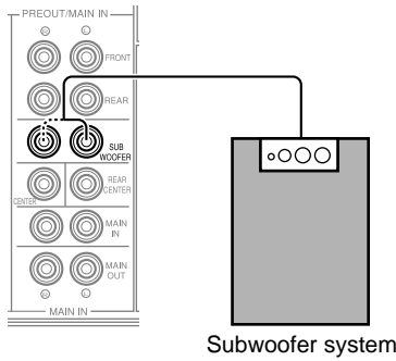
Subwoofer system
