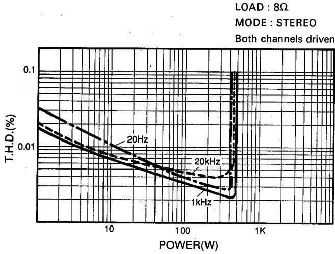
T.H. DISTORTION VS. OUTPUT POWER
