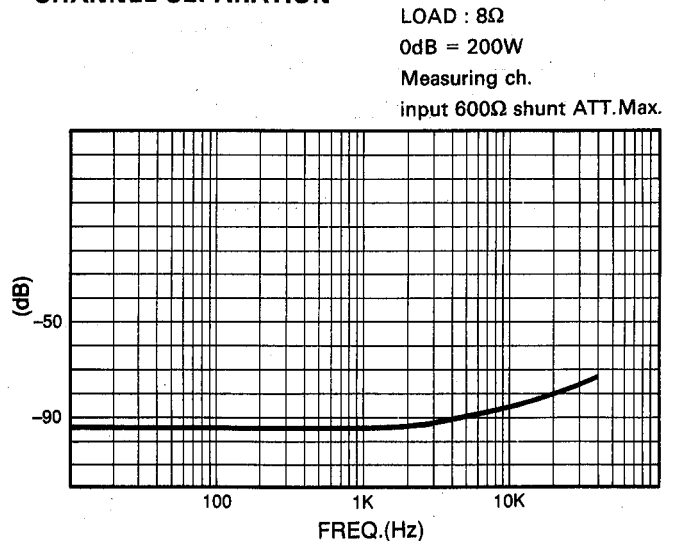
CHANNEL SEPARATION
