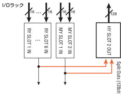
Conceptual diagram of recording system for a virtual sound check (an example)
